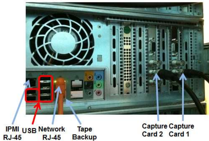
Figure: Typical server rear panel
