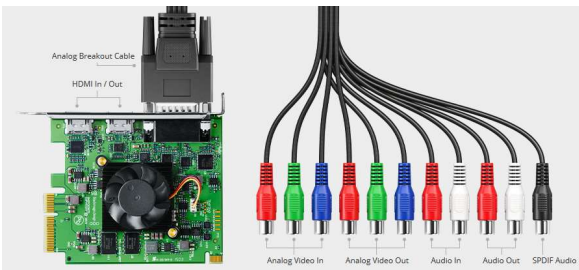
Figure: Intensity Pro & breakout cable
