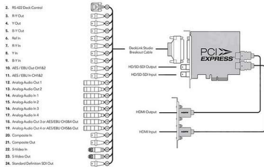
Figure: DeckLink Studio connections
