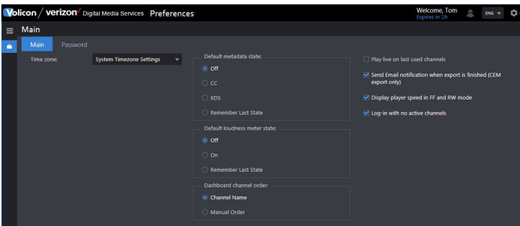
Figure: Preferences
