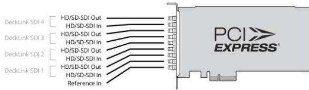
Figure: DeckLink Quad SDI-SD/HD connector diagram
