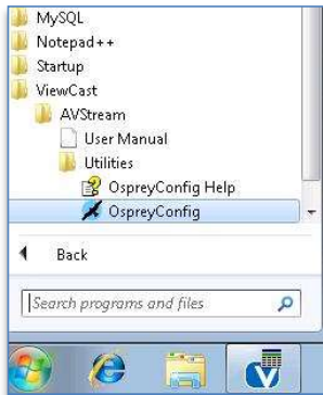
Figure: OspreyConfig
