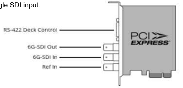
Figure: DeckLink SDI connector connections
