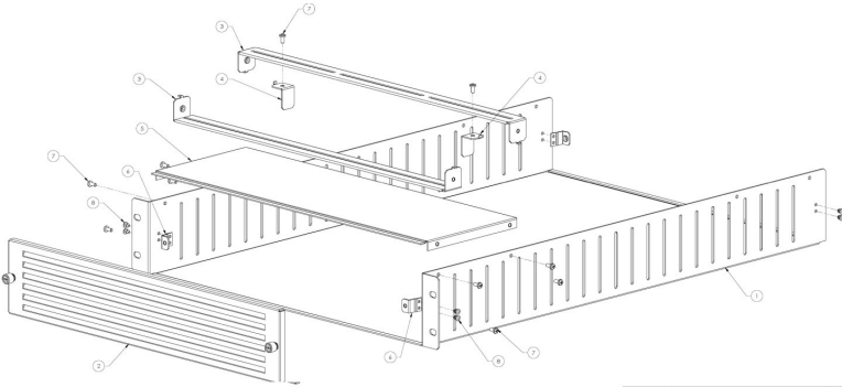
Figure: Set-top box mounting shelf
